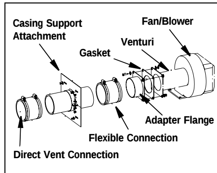
Figure B6-21. Air Inlet Extension kit for Direct Vent combustion
